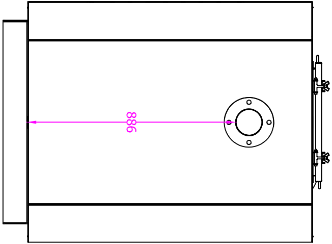
OUTLET SIDE
