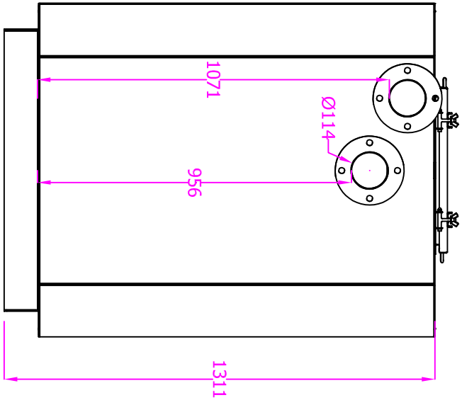
INLET SIDE
